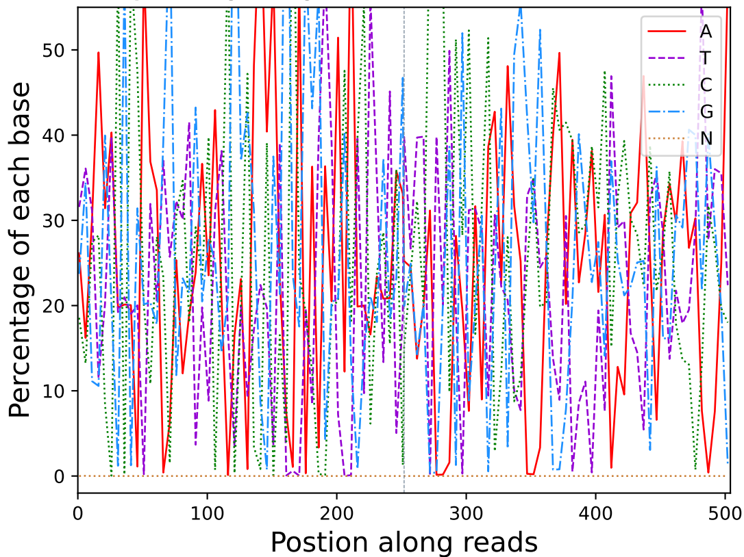
Base percentage along reads (R20221)
